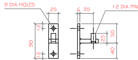
4 x GATE HINGE
